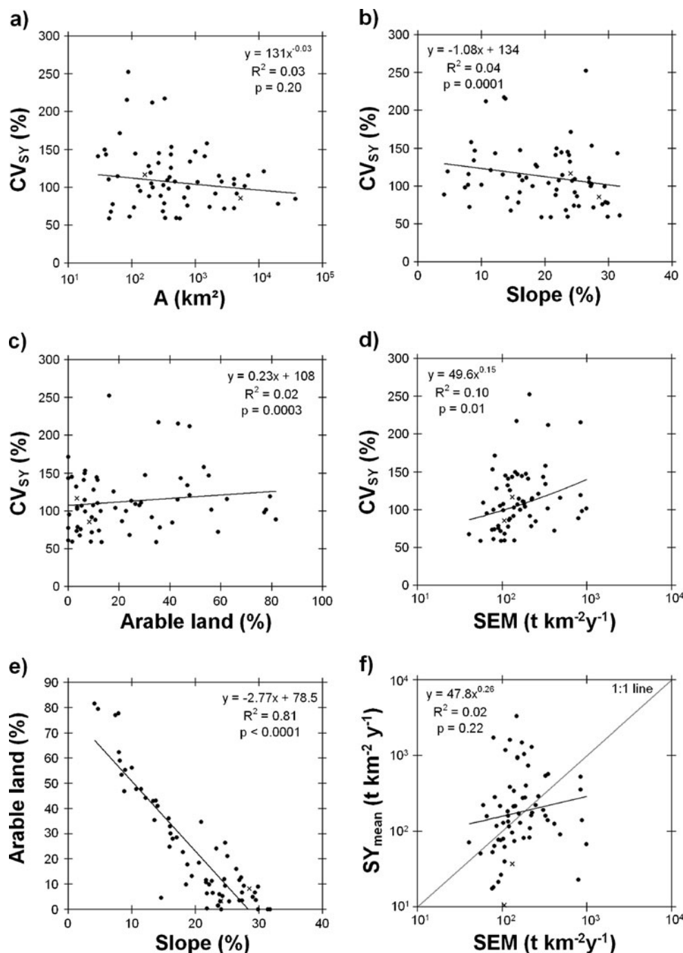
Fig. 9 Relationships between the coefficients of variation of annual sediment yield ( CV_{SY} ) and various catchment characteristics for 65 sub-catchments of the Siret basin in Romania (see Fig. 1). The two catchments indicated with an x are affected by dams and were not included in the regression analyses. All regressions are therefore based on 63 observations (representing 2,477 catchment-years of observations). A catchment area, Slope estimated average slope of the catchment, Arable\ land estimated aerial fraction of arable land, SEM estimated average sheet and rill erosion rate according to the map of Cerdan et al. (2010), SY_{mean} average annual sediment yield for the whole measuring period
